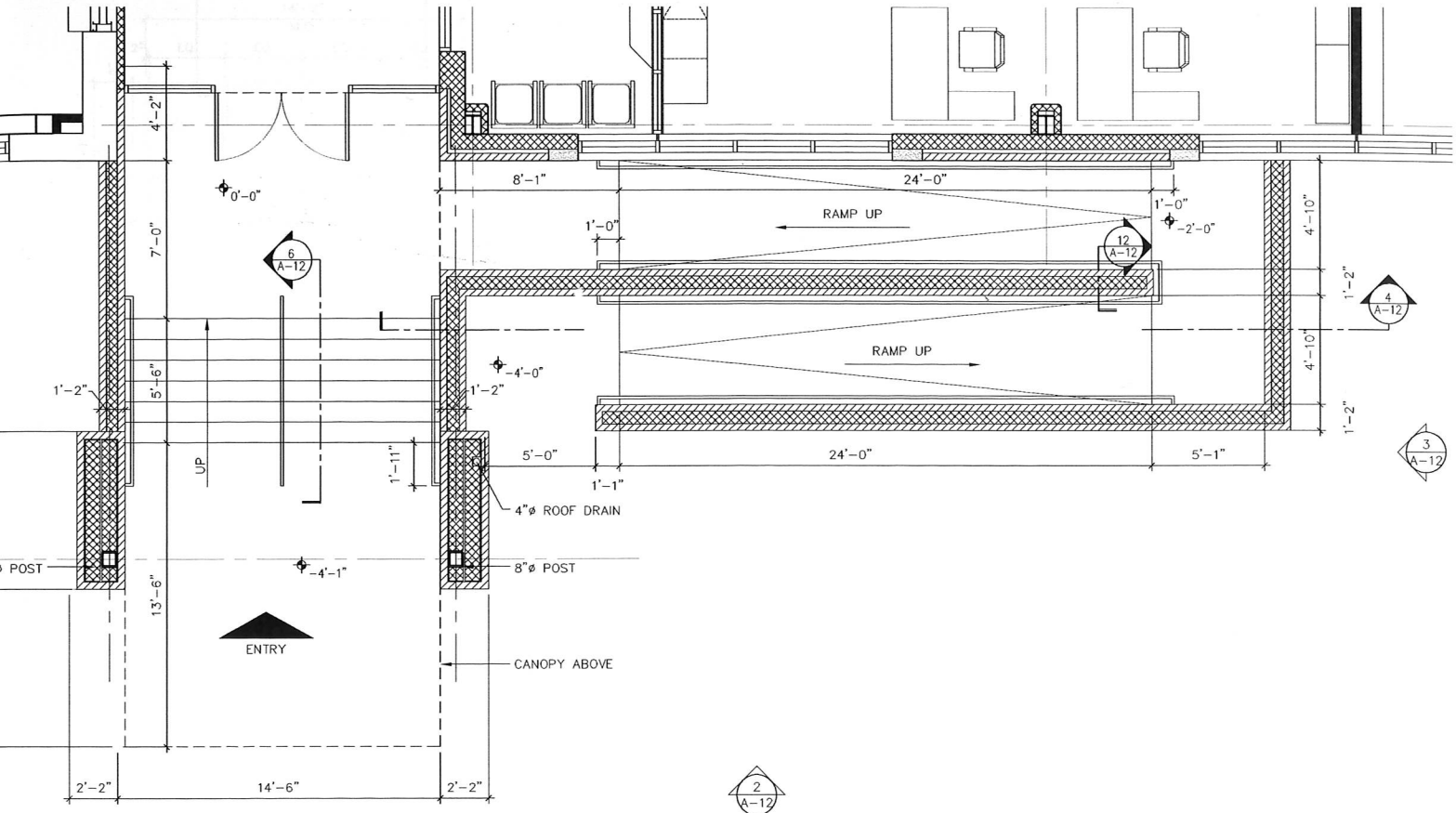
1 ENLARGED PLAN A-12 @ STAIR, RAMP AND CANOPY 1/4"=1'-0"
