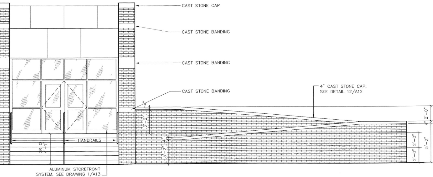
2 ELEVATION A-12 1/4"=1'-0"
